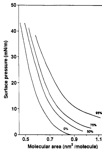
FIGURE 3: Compression isotherms of mixed films. Detergent/phospholipid mixtures were spread at the indicated relative content in CTAB. Each compression isotherm has been reproduced three times.
